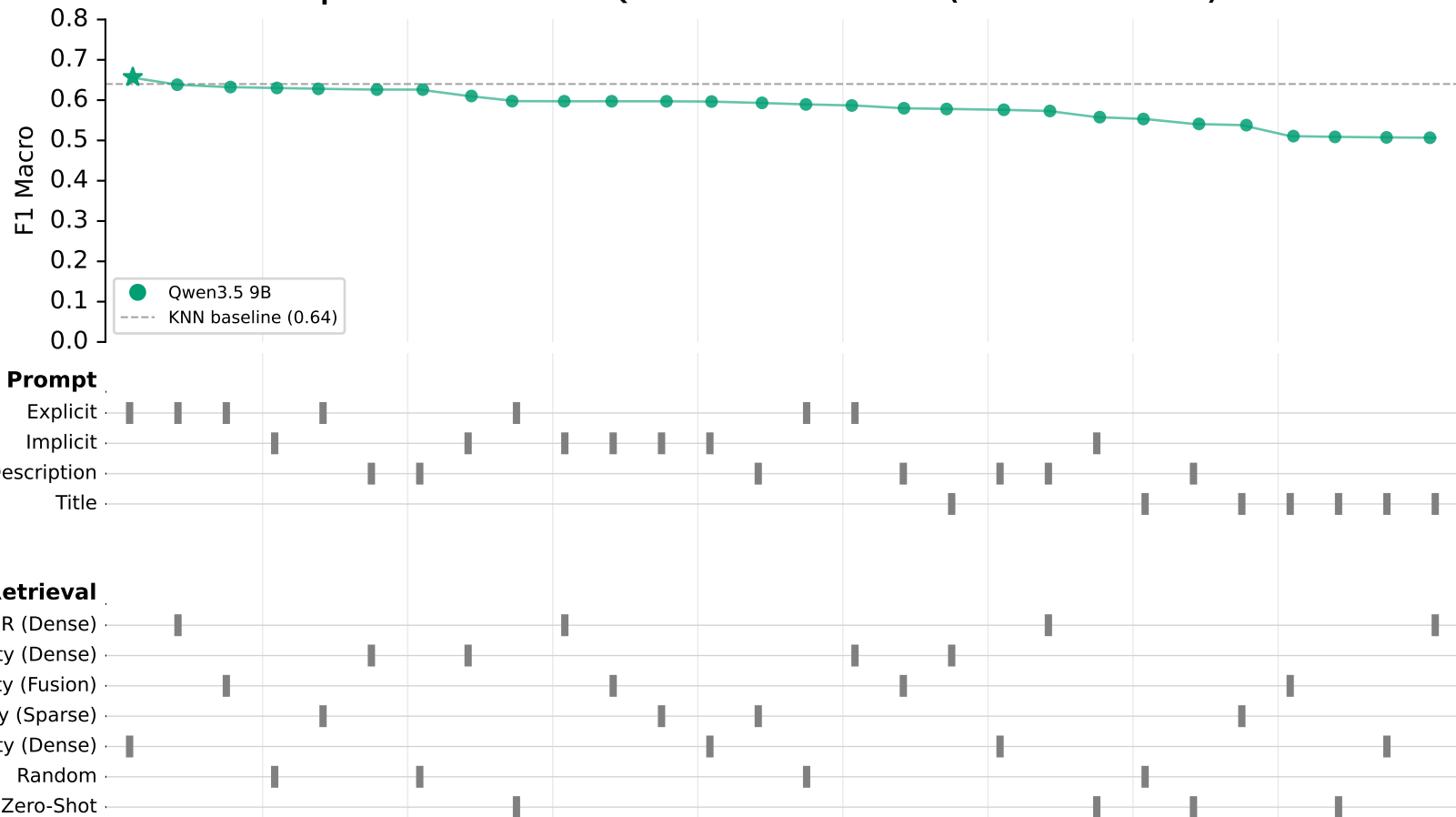
Specification Curve — Qwen3.5 9B — F1 Macro (mean across folds)
